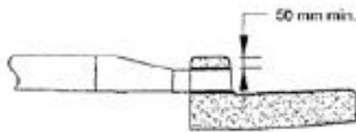
UPVC PIPE/ ADAPTOR AND RHS KERB FITTING
