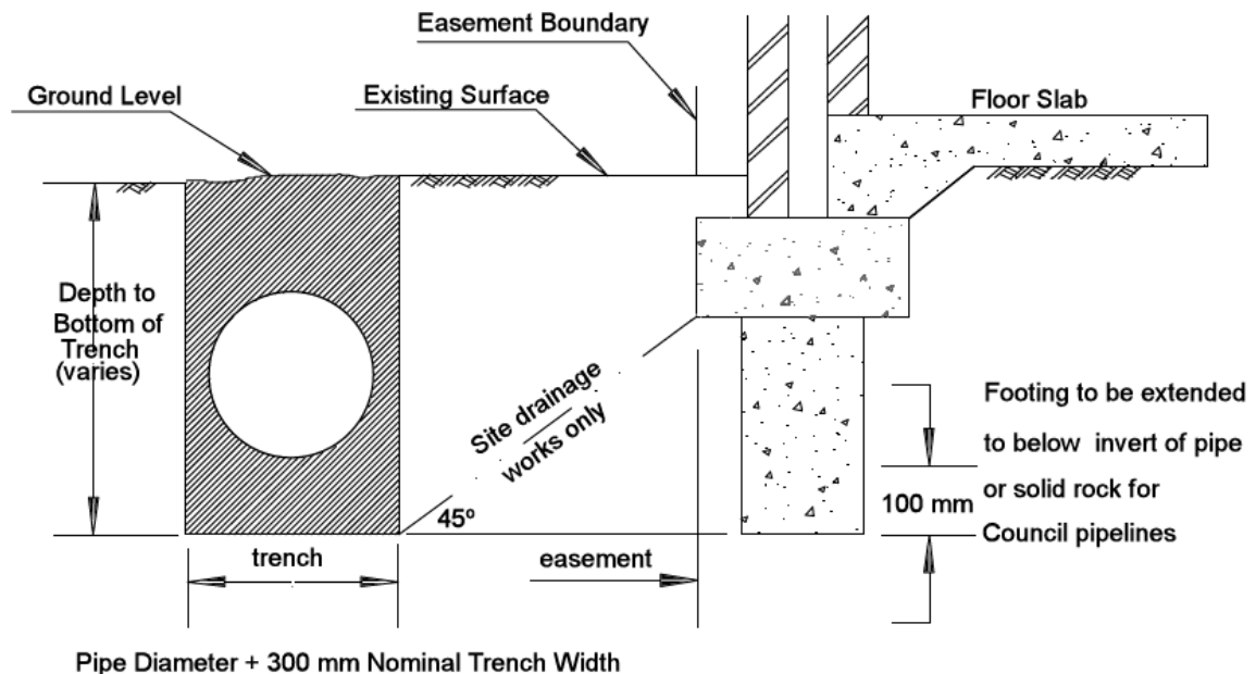
Figure 1-11 - Drainage easement adjacent to a building.
