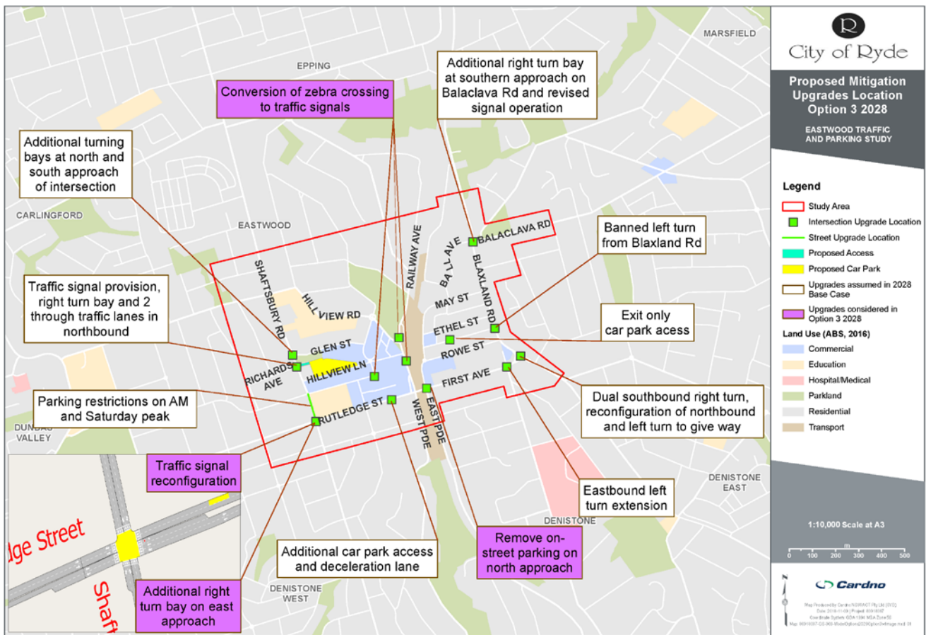
Figure 5-9 Option 3 Road Network Upgrades
