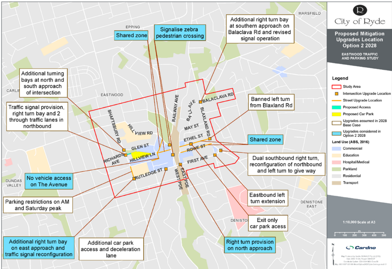
Figure 5-6 Option 2 Road Network Upgrades
