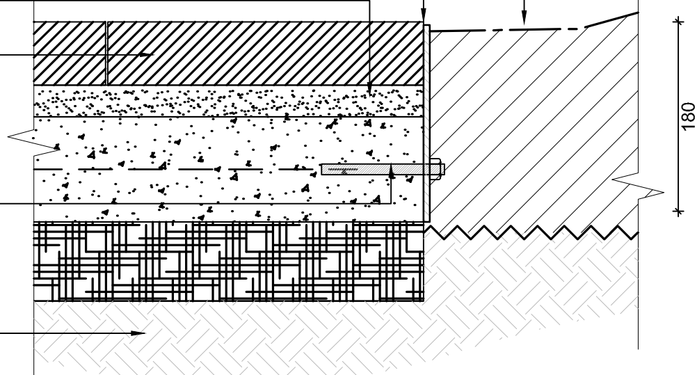
PV 6.2 STEEL FLAT TO CURVED GARDEN BED EDGE - TYPICAL SCALE 1:5 AT A4
