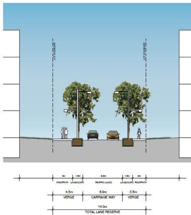
Figure 4.1.3 14m Wide Streets – Typical section
