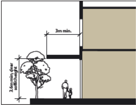
Figure 7.4.1 Awnings: Section
