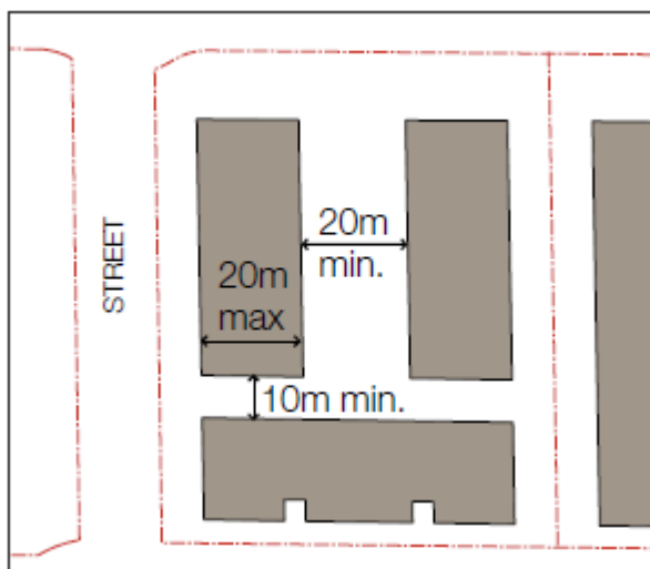
Figure 7.7.1 Commercial Building separation controls
