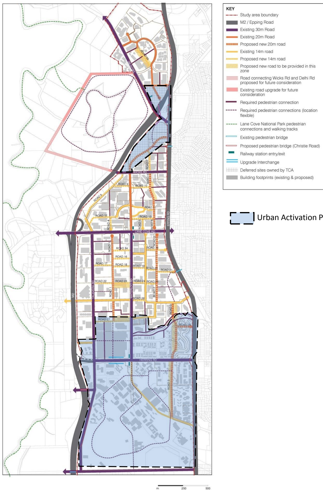
Figure 4.1.1 Access Network
