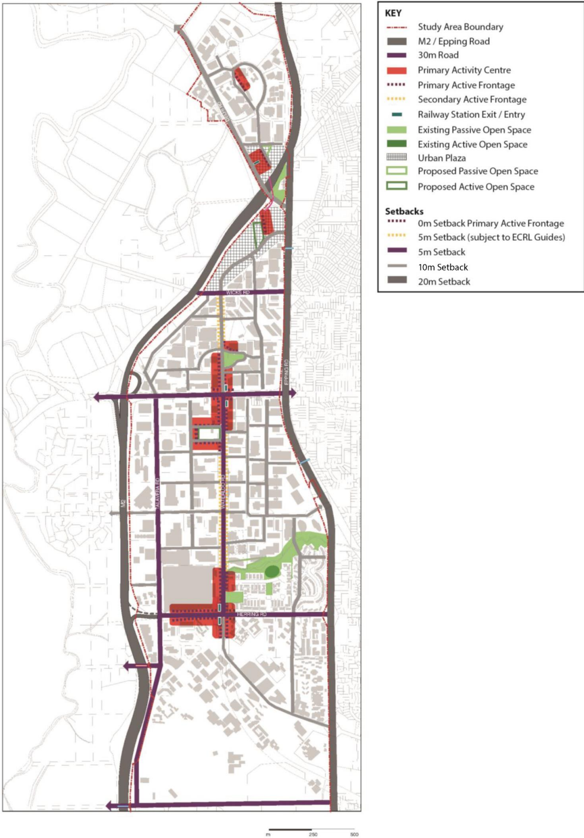
Figure 7.3.1 Setback Control Drawing
