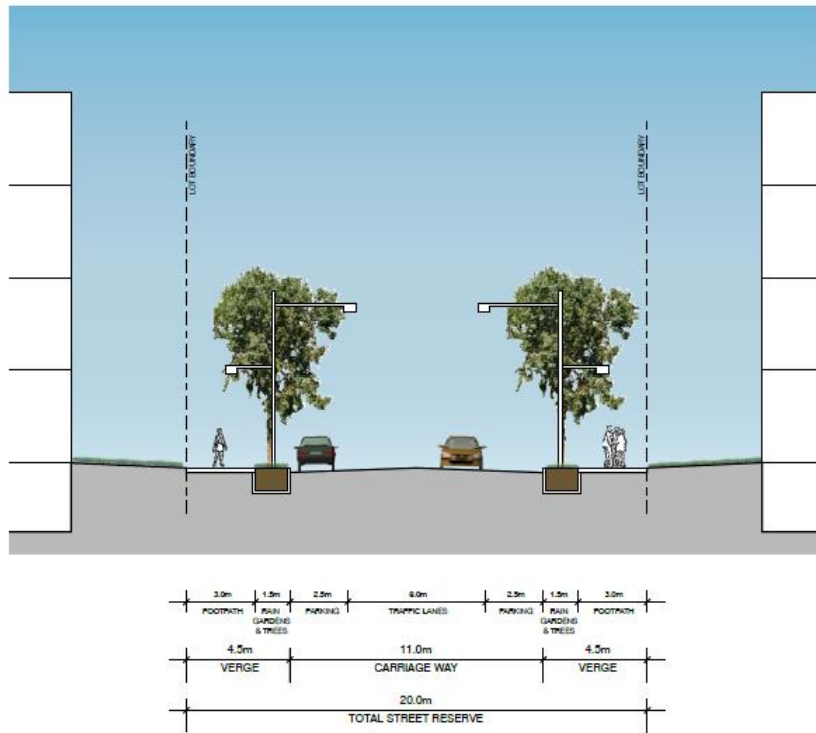
Figure 4.1.2 20m Wide Streets – Typical section
