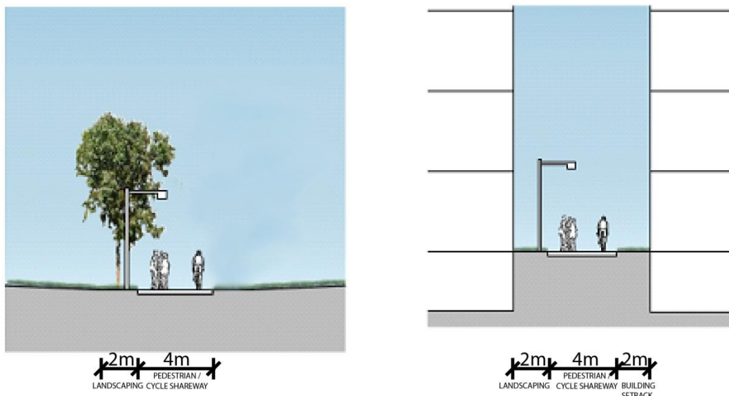
Figure 4.2.1 Pedestrian Ways Typical sections
