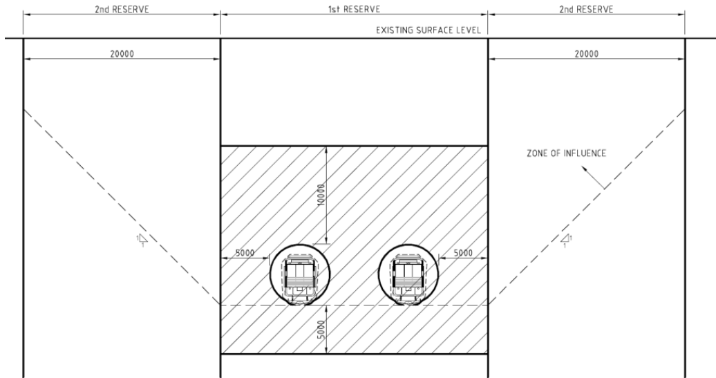
Figure 7.2.3 Section showing First and Second Reserve Zones associated with ECRL underground rail infrastructure in Macquarie Park Corridor
