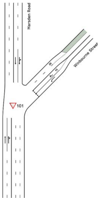
Figure 4.2: Intersection 2: Marsden Road / Winbourne Street SIDRA Layout
