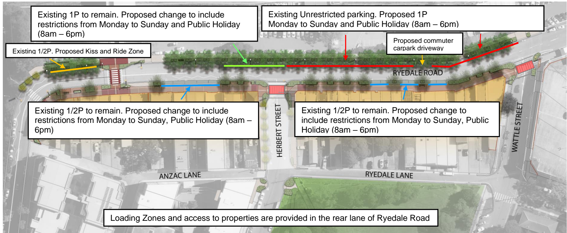
Figure 1 Proposed Parking changes on Ryedale Road, West Ryde.
