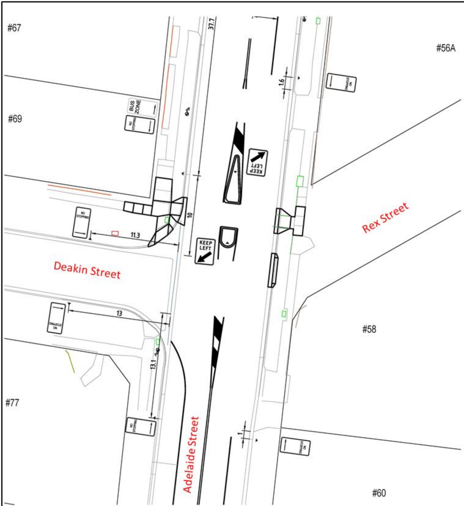
PLAN SCALE 1:200 AT A1
