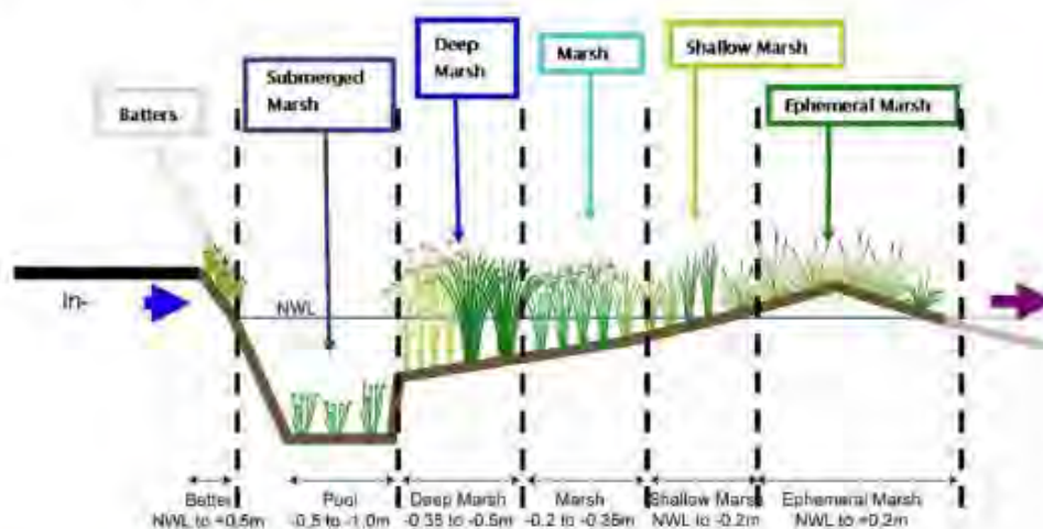
Wetland Long Section (indicative only)
