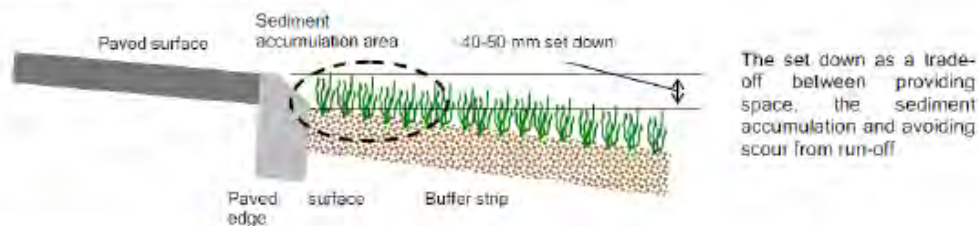
Figure 12: Typical buffer strip arrangement
