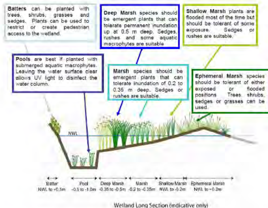
Figure 25 – Indicative wetland long section showing plant zones.
