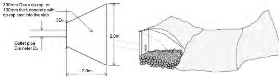
Figure 1-2 Outflow apron.
