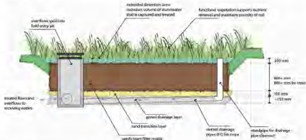
Figure 15: Bioretention system typical arrangement
