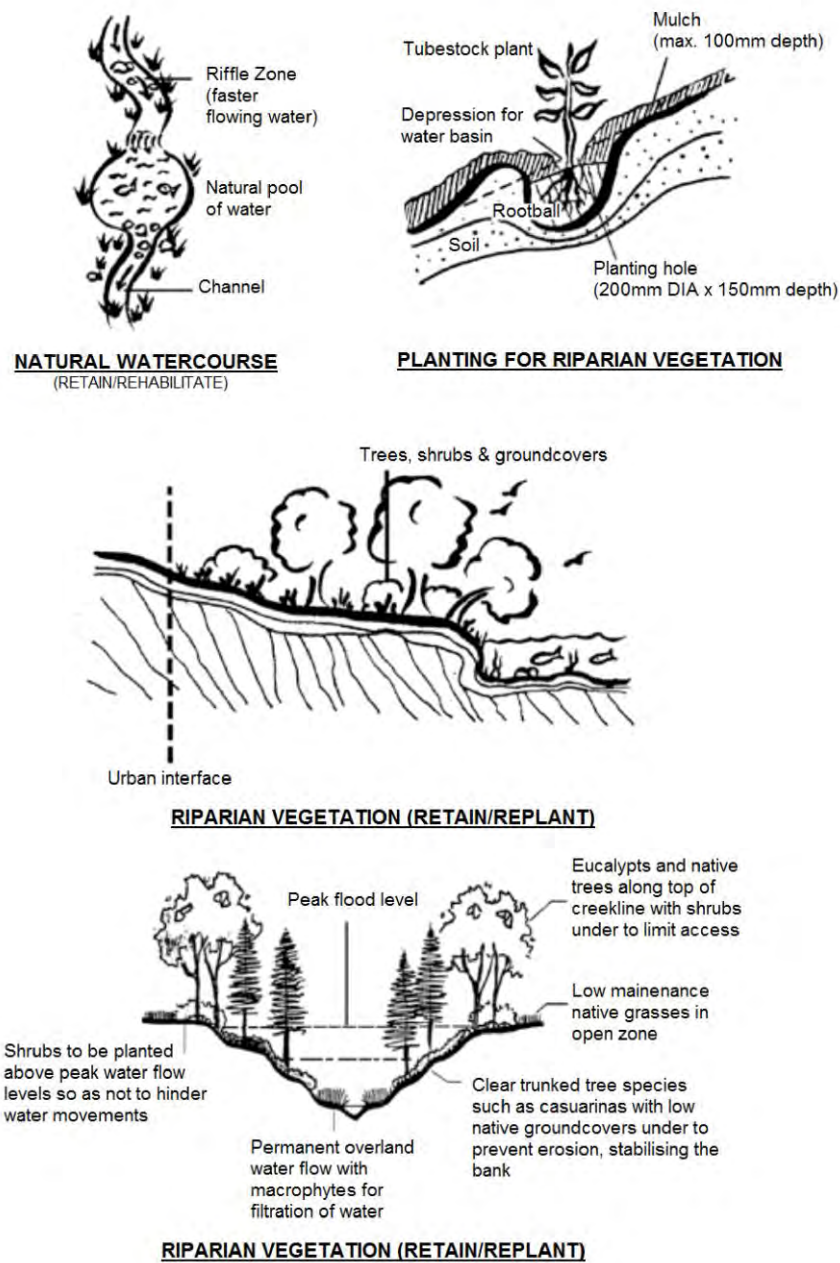
Figure 6-1: Examples of Riparian Systems
