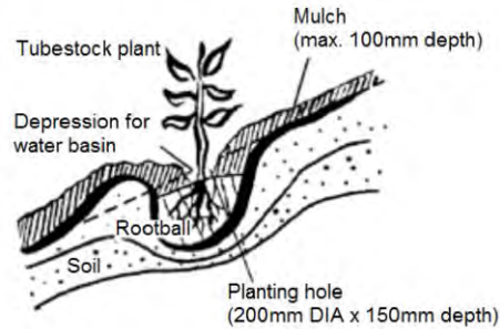
PLANTING FOR RIPARIAN VEGETATION
