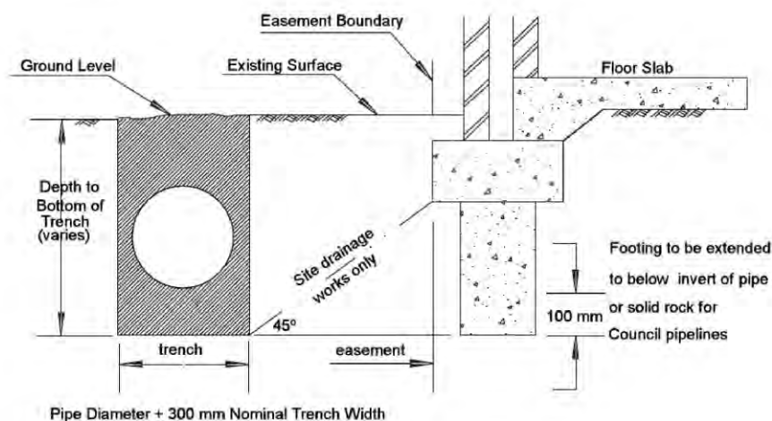
Figure 1-11 - Drainage easement adjacent to a building.
