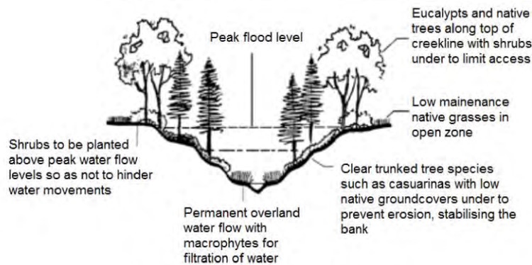
RIPARIAN VEGETATION (RETAIN/REPLANT)
