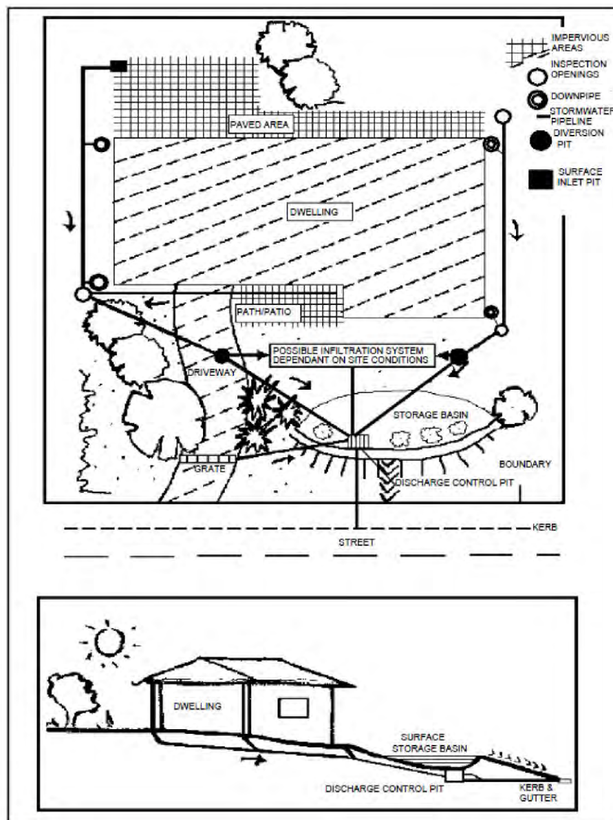
Figure 1-7 : Simplified Above Ground Storage System
