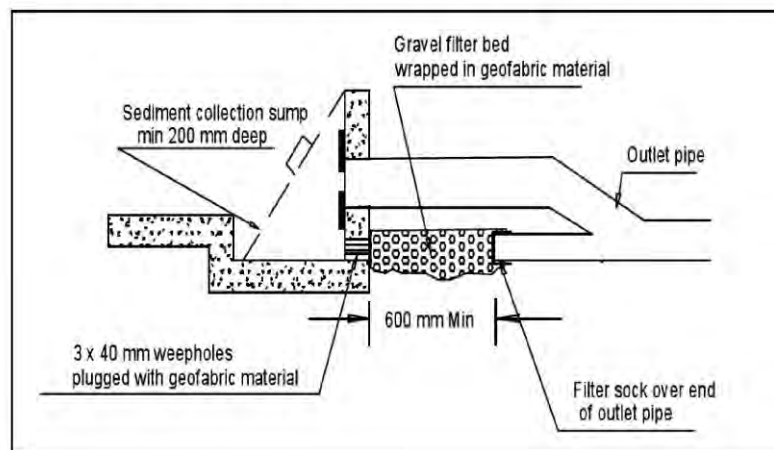
Figure 1-9 - Typical sediment collection sump.
