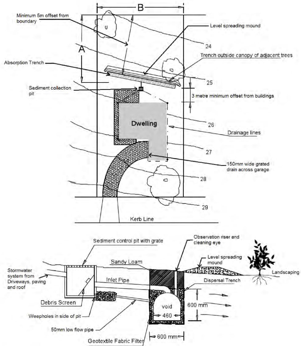
Figure 1-5: Typical Absorption System layout
