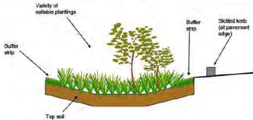
Figure 9 – Typical swale arrangement.
