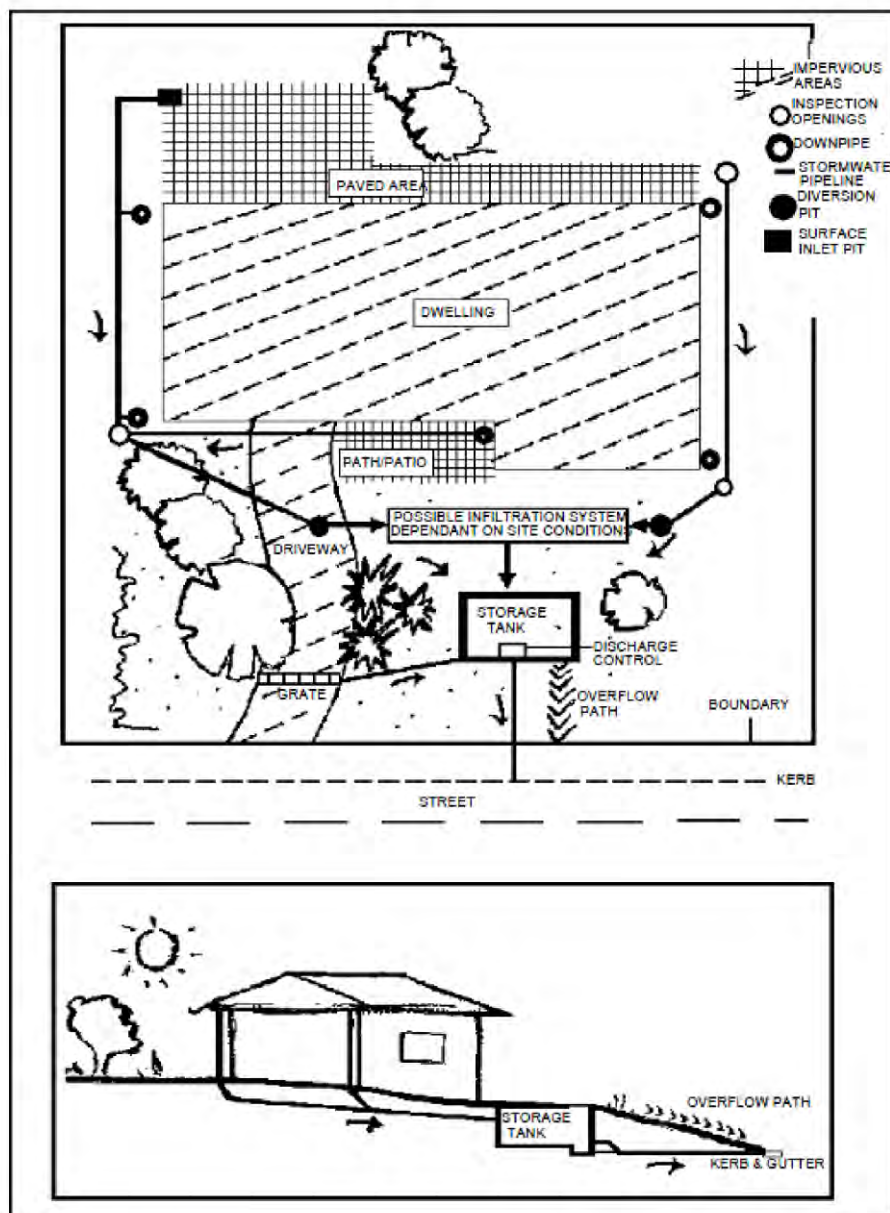
Figure 1-6 : Simplified Below Ground Storage System
