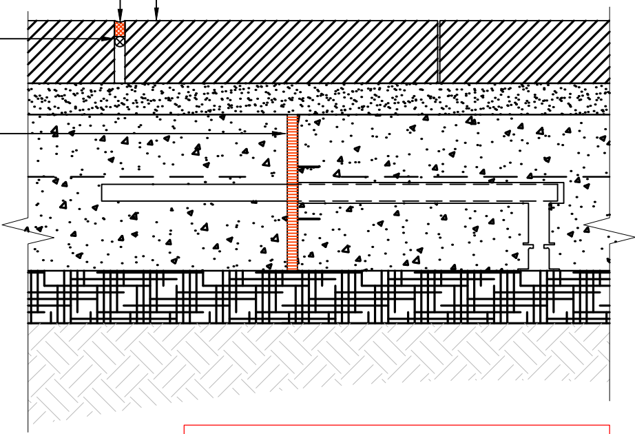
PV 3.1.1 GRANITE EXPANSION JOINT (EJ) SCALE 1:5 AT A4
