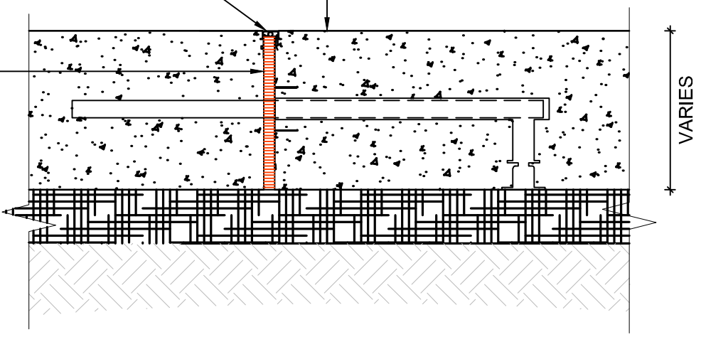
PV 3.1 CONCRETE EXPANSION JOINT (EJ) - TYPICAL SCALE 1:5 AT A4
