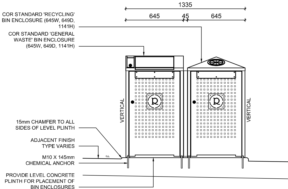
SF RUBBISH BIN INSTALLATION - TYPICAL ELEVATION 4.0 SCALE 1:20 AT A4
