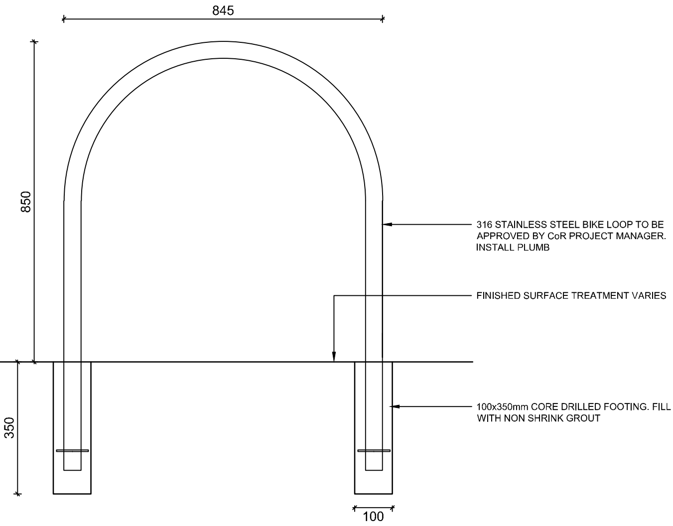
SF 5.1 STAINLESS STEEL BIKE LOOP - TYPICAL SCALE 1:10 AT A4
