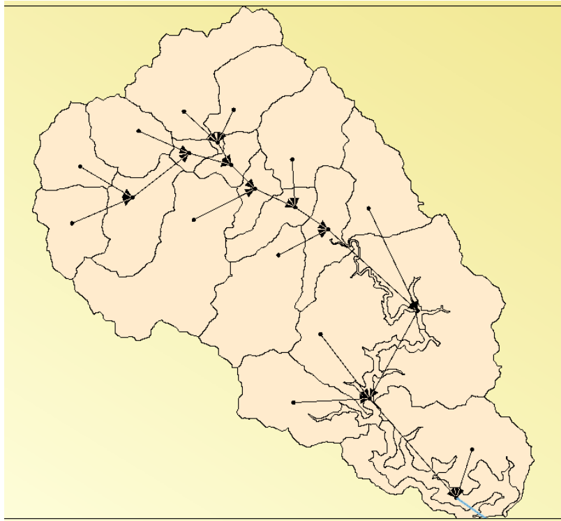
Figure 3-1: Lane Cove River catchment runoff model built in Source Catchments
