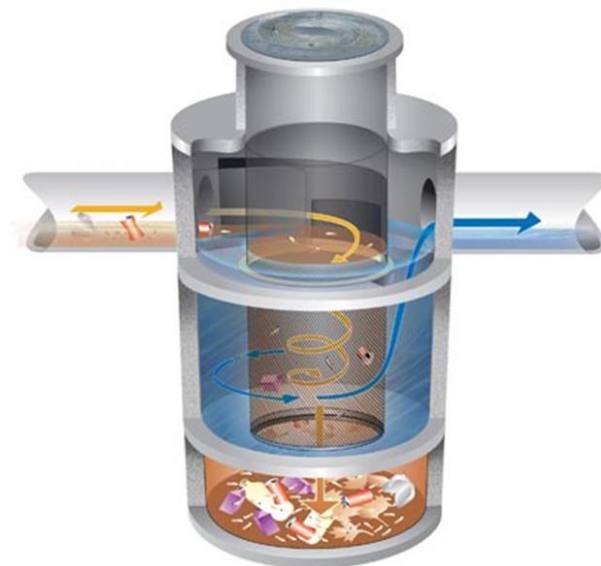
Figure 12-3: Gross Pollutant Trap Schematic 14
