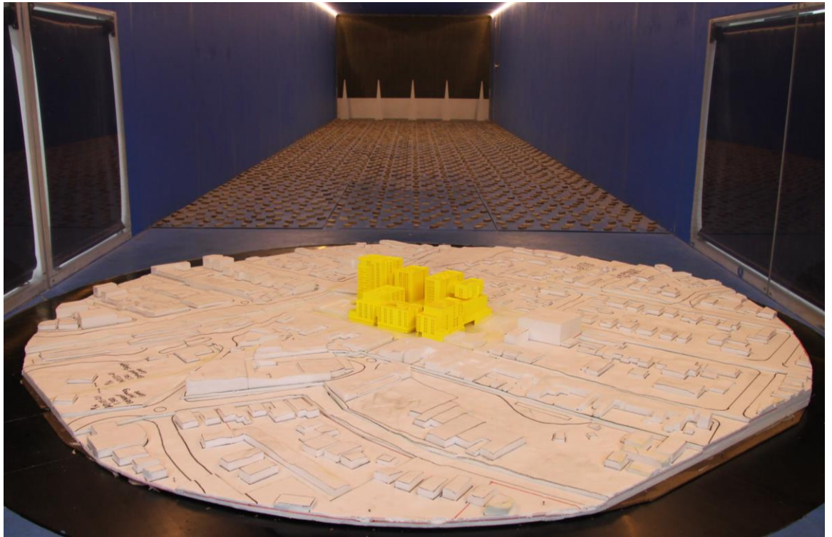
Figure 2d: Photograph of the Wind Tunnel Model (view from the north-west)
