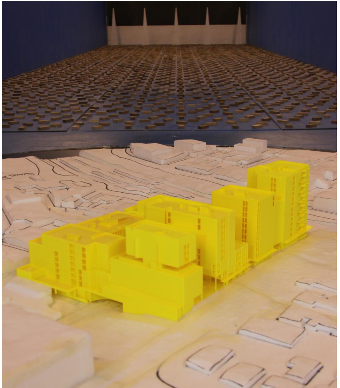
Figure 2f: Photograph of the Wind Tunnel Model (view from the south-west)
