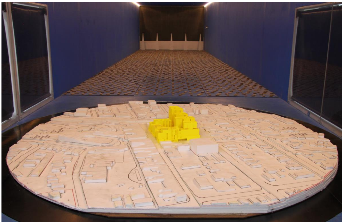
Figure 2e: Photograph of the Wind Tunnel Model (view from the west)
