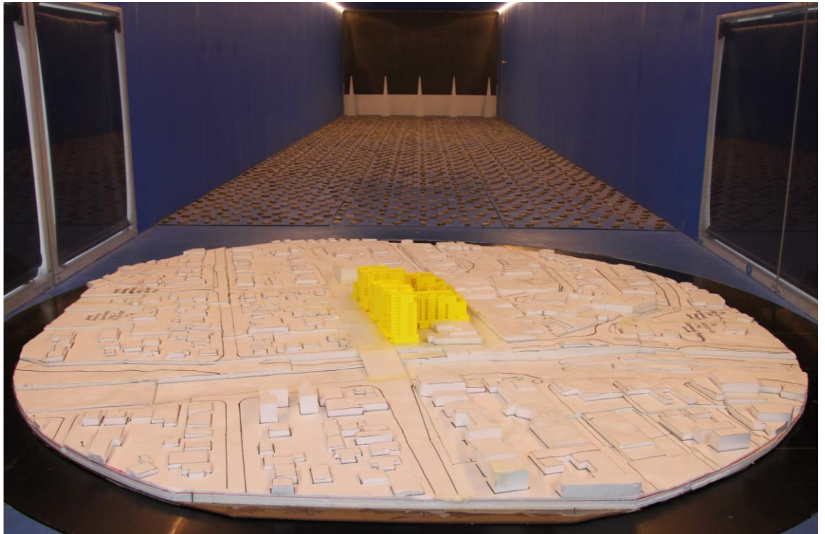
Figure 2b: Photograph of the Wind Tunnel Model (view from the east)
