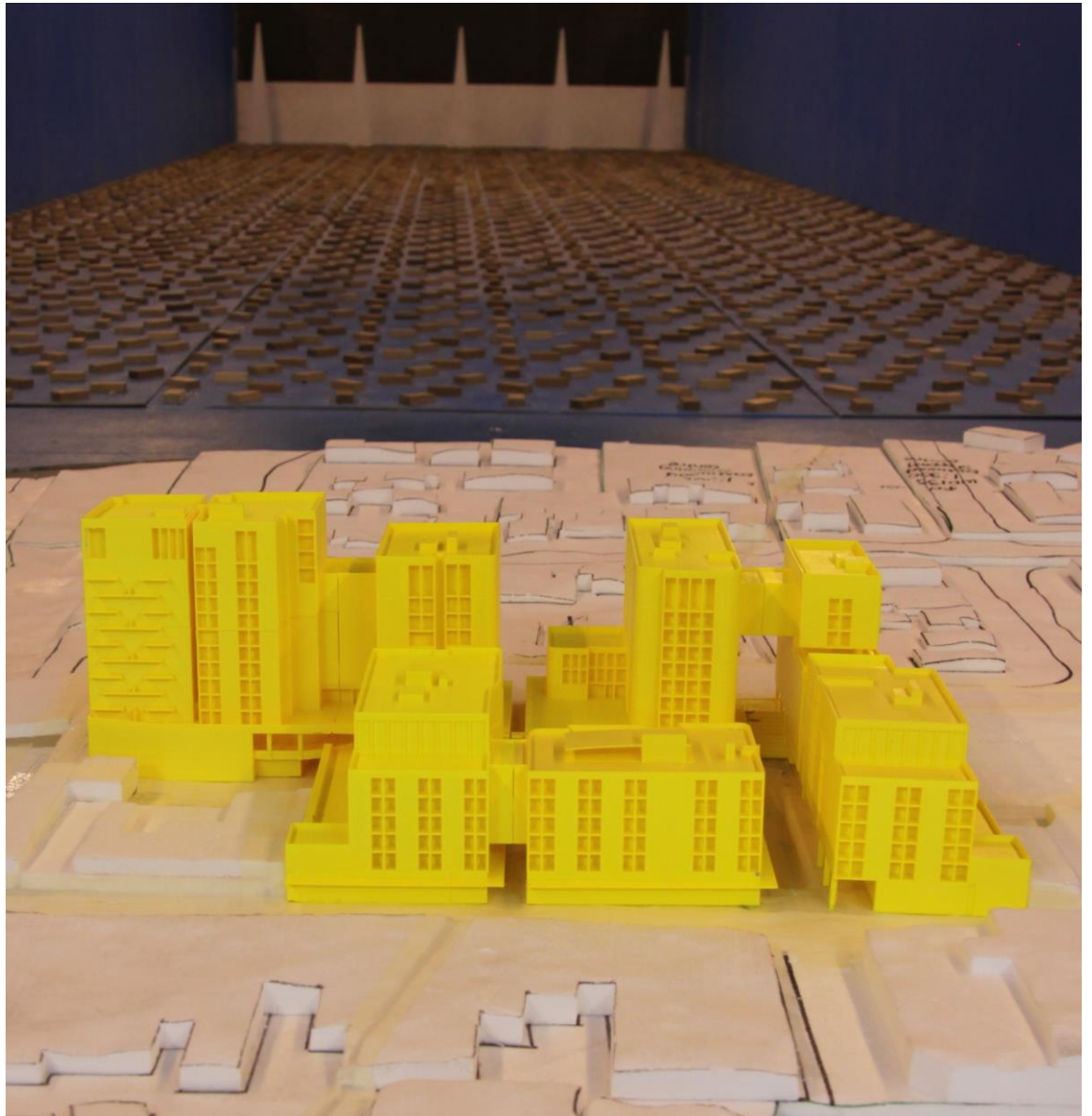
Figure 2g: Photograph of the Wind Tunnel Model (view from the north-east)
