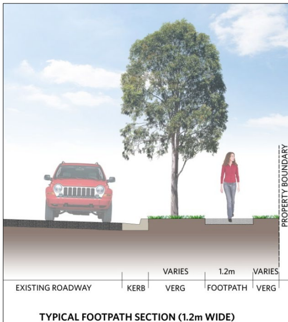
TYPICAL FOOTPATH SECTION (1.2m WIDE)
