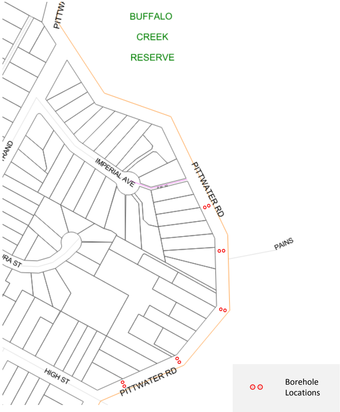
PITTWATER ROAD (Western side from High St to Field of Mars) EXTENT OF PAVEMENT INVESTIGATION WORKS
